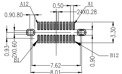
RECOMMENDED PCB LAYOUT( \pm 0.80 \pm 0.05 ) COMPONENT SIDE(GENERAL TOLERANCE: \pm 0.05 )
