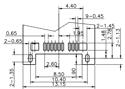
RECOMMENDED P.C.B. LAYOUT TOLERANCE UNSPECIFIED ±0.05mm
