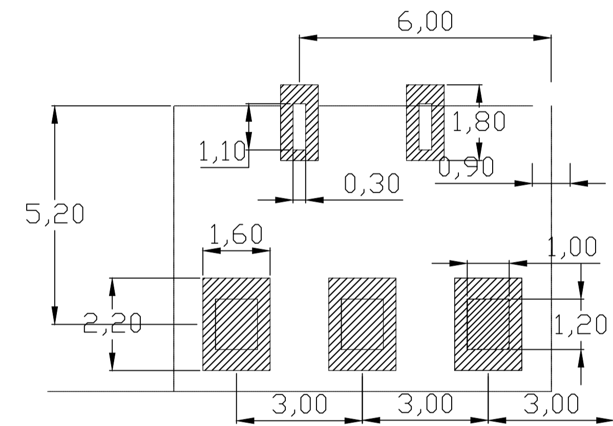
RECOMMENDED PCB LAYOUT TOP VIEW (.XX±0.05)
